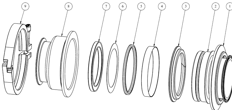
Clamp Style End Connection Shown
