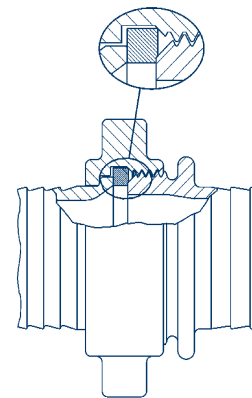
washer seal
